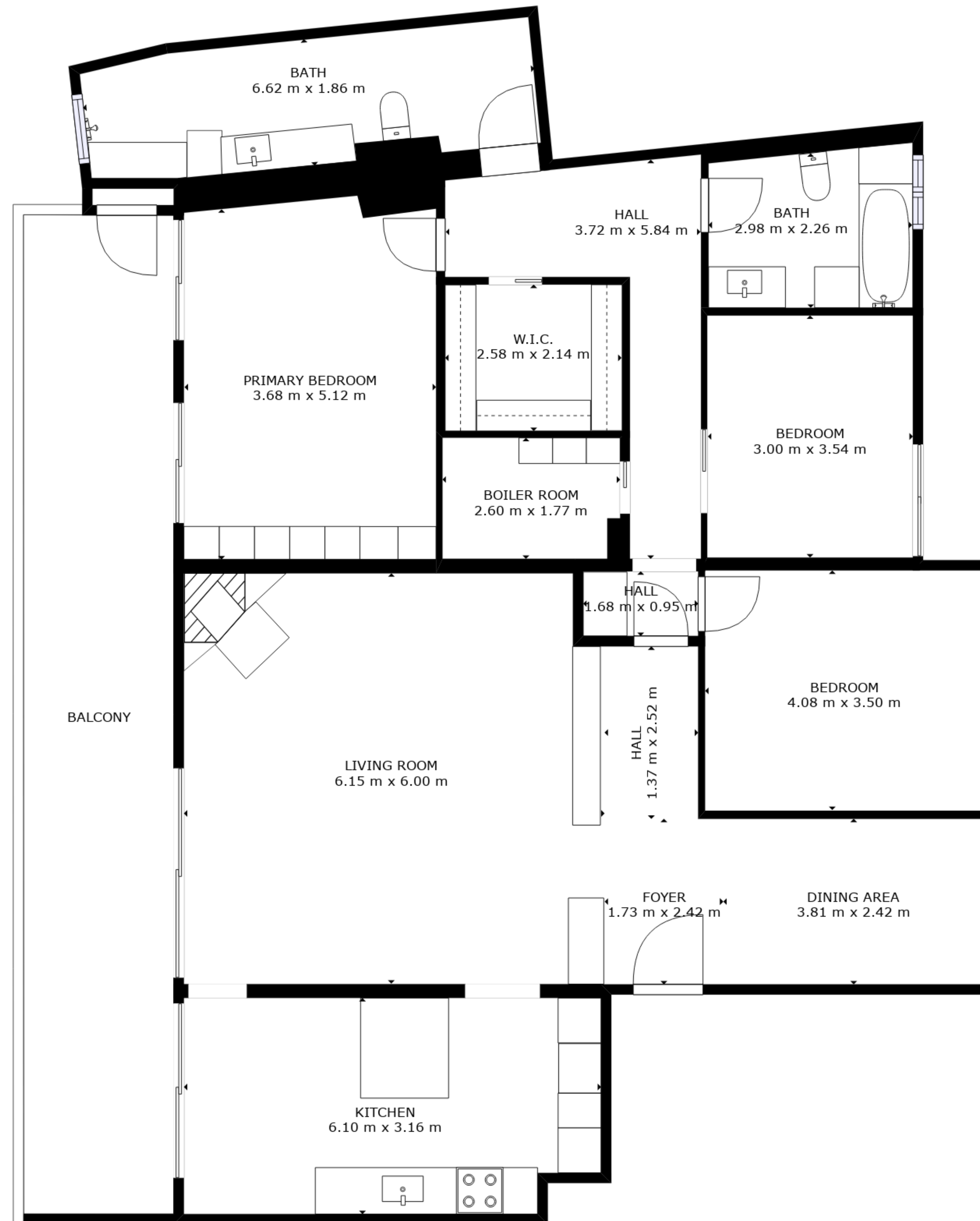
FLOOR 1
